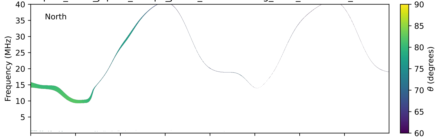
expres_earth_jupiter_europa_jrm33_lossc-wid1deg_3kev_20121021_v11.cdf
