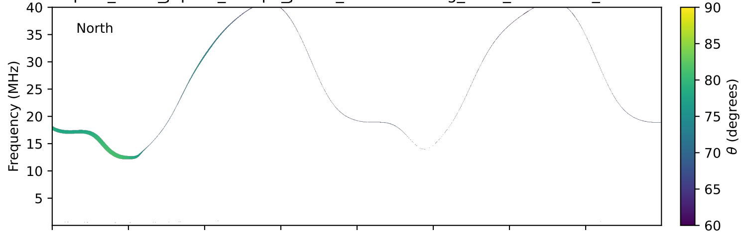
expres_earth_jupiter_europa_jrm33_lossc-wid1deg_3kev_20121014_v11.cdf
