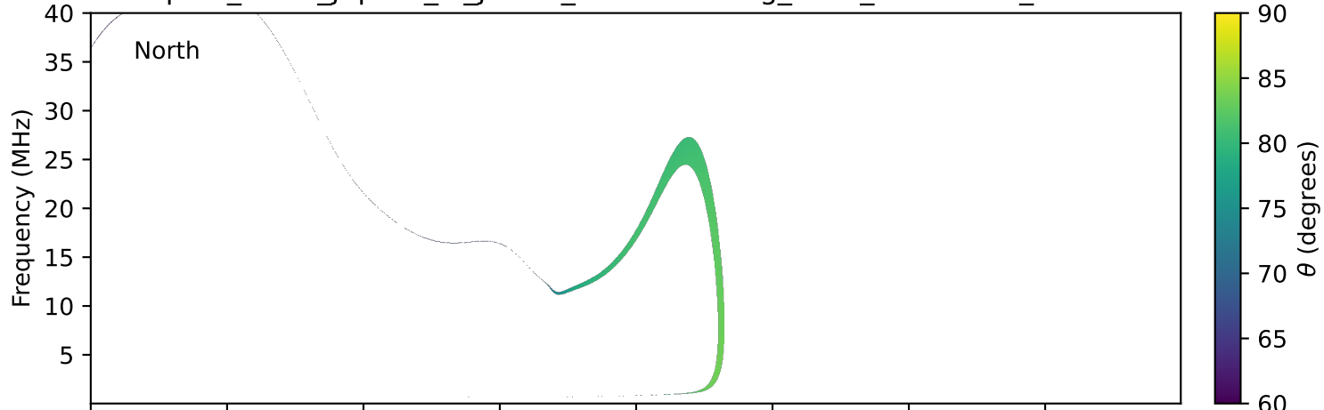
expres_earth_jupiter_io_jrm33_lossc-wid1deg_3kev_20120824_v11.cdf
