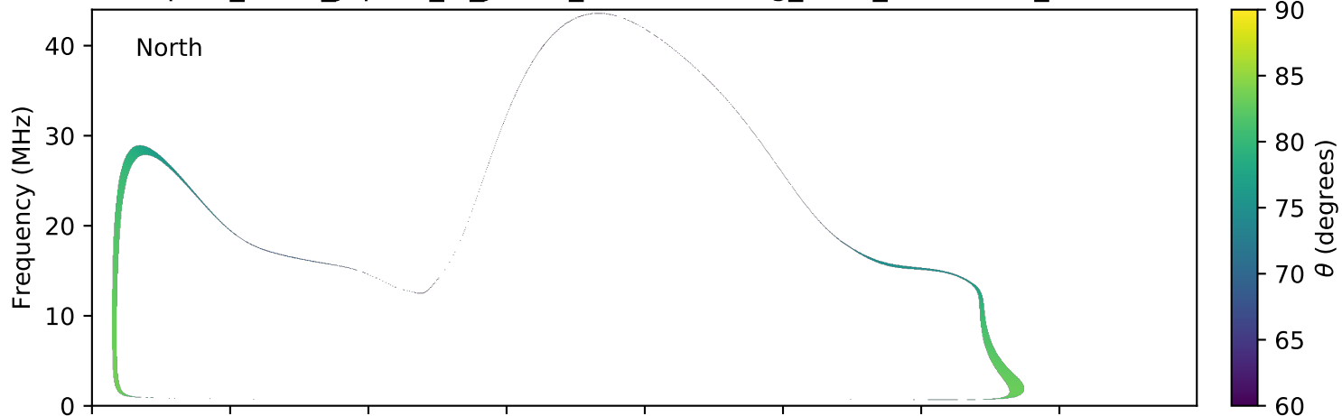
expres_earth_jupiter_io_jrm09_lossc-wid1deg_3kev_20120829_v01.cdf
