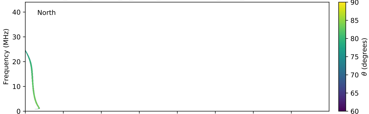
expres_earth_jupiter_io_jrm09_lossc-wid1deg_3kev_20120828_v01.cdf
