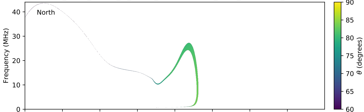
expres_earth_jupiter_io_jrm09_lossc-wid1deg_3kev_20120824_v01.cdf
