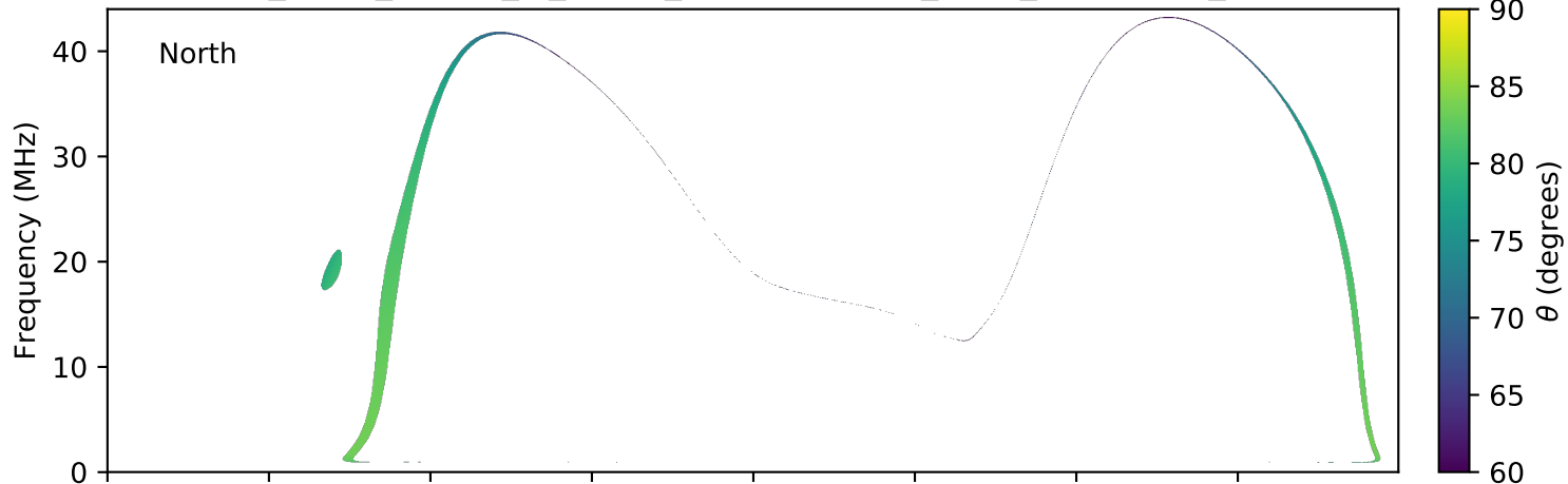
expres_earth_jupiter_io_jrm09_lossc-wid1deg_3kev_20120820_v01.cdf
