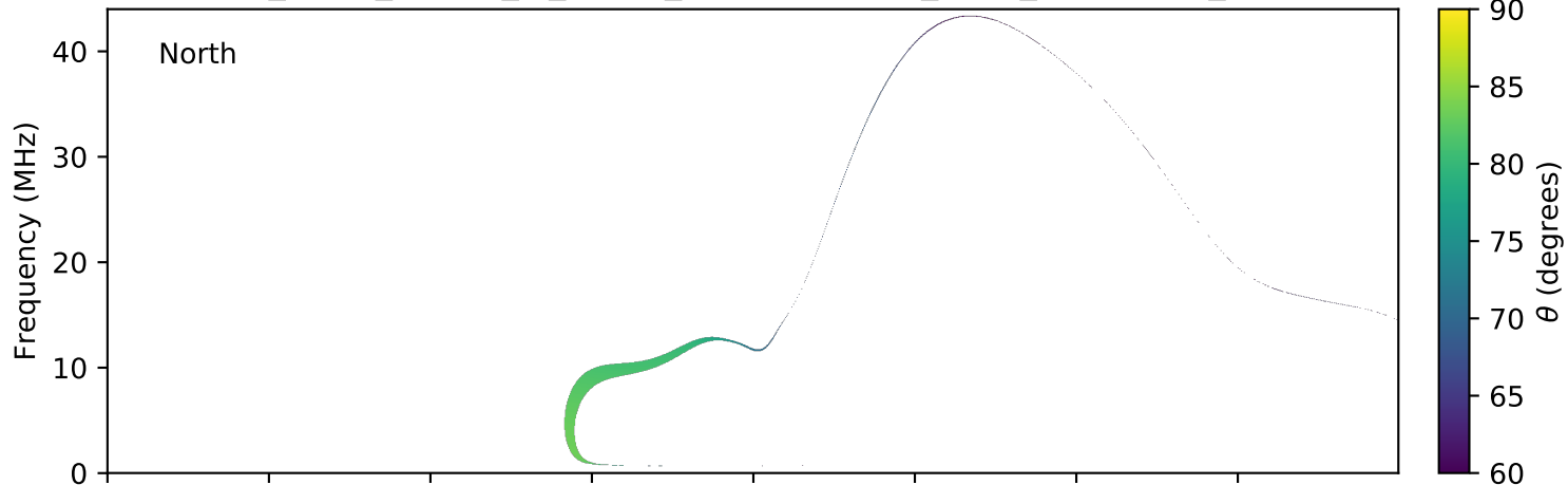
expres_earth_jupiter_io_jrm09_lossc-wid1deg_3kev_20120818_v01.cdf
