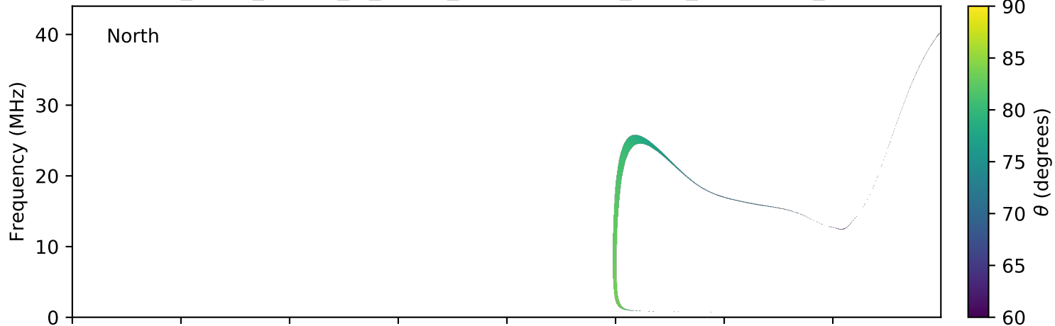
expres_earth_jupiter_io_jrm09_lossc-wid1deg_3kev_20120816_v01.cdf
