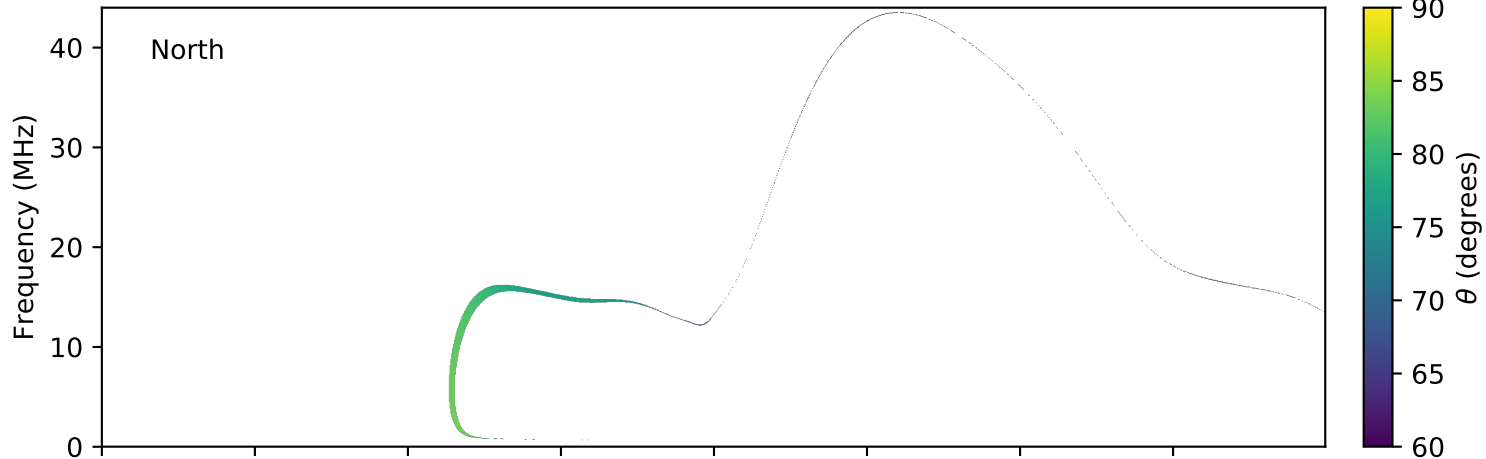
expres_earth_jupiter_io_jrm09_lossc-wid1deg_3kev_20120811_v01.cdf
