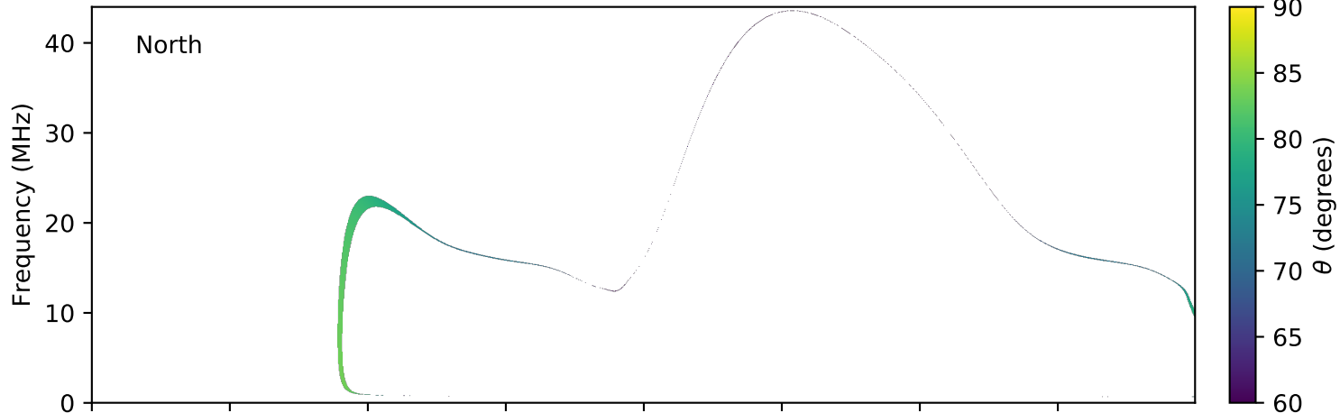
expres_earth_jupiter_io_jrm09_lossc-wid1deg_3kev_20120804_v01.cdf
