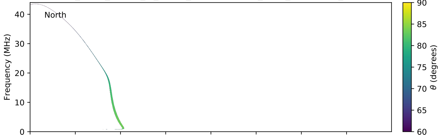
expres_earth_jupiter_io_jrm09_lossc-wid1deg_3kev_20120803_v01.cdf
