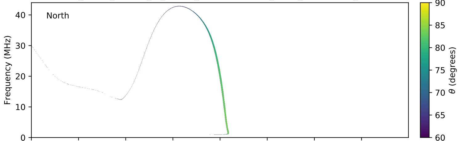
expres_earth_jupiter_io_jrm09_lossc-wid1deg_3kev_20120801_v01.cdf
