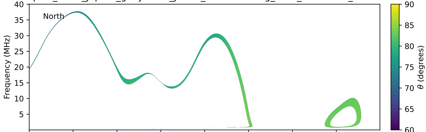
expres_earth_jupiter_ganymede_jrm33_lossc-wid1deg_3kev_20120829_v11.cdf
