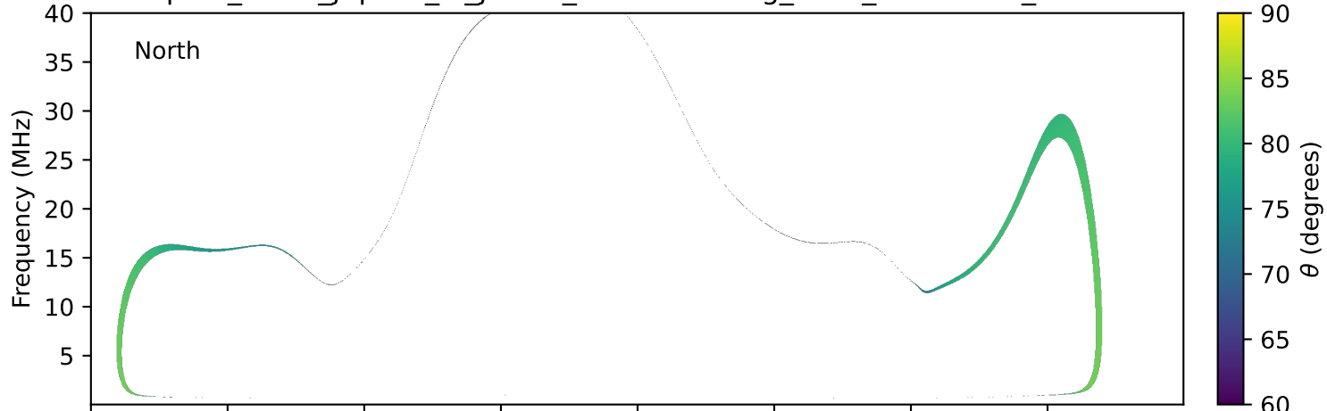
expres_earth_jupiter_io_jrm33_lossc-wid1deg_3kev_20120628_v11.cdf
