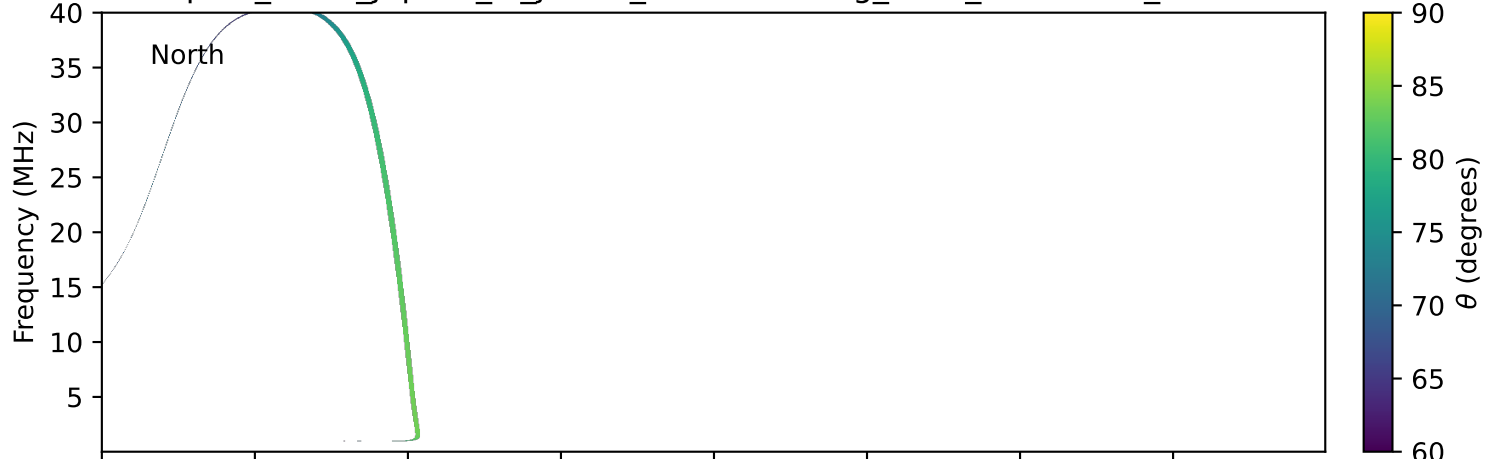
expres_earth_jupiter_io_jrm33_lossc-wid1deg_3kev_20120618_v11.cdf
