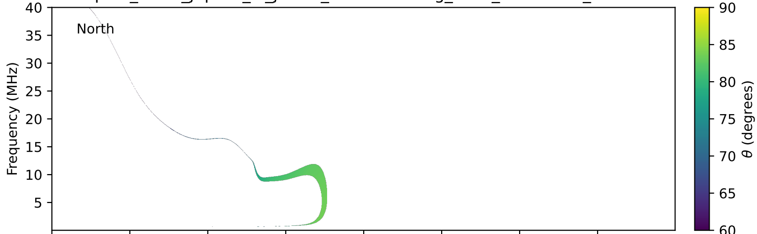
expres_earth_jupiter_io_jrm33_lossc-wid1deg_3kev_20120609_v11.cdf
