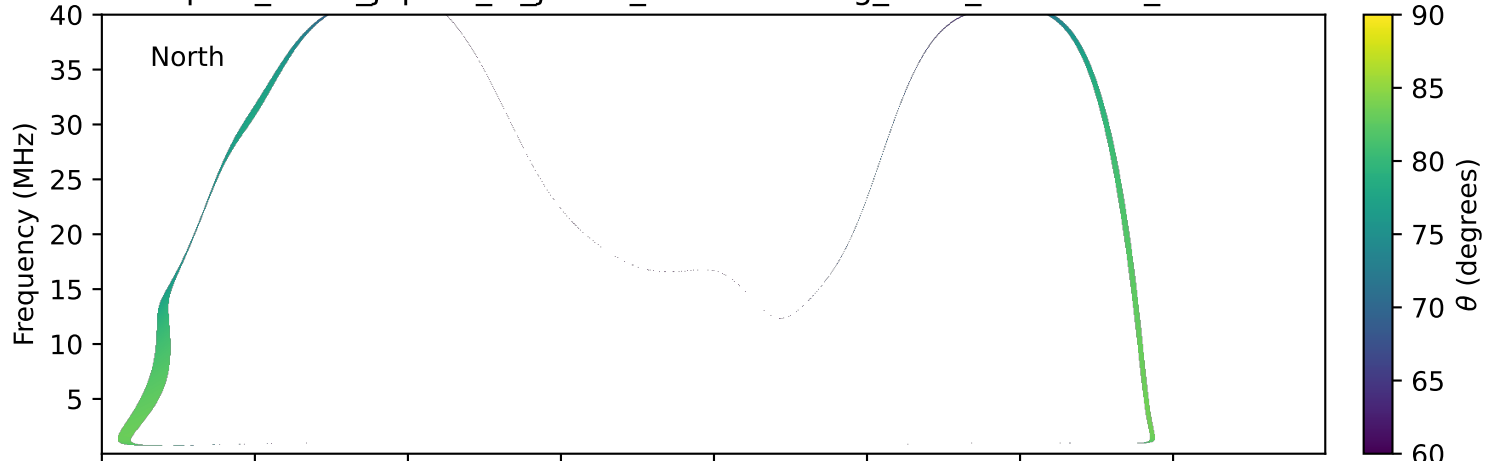
expres_earth_jupiter_io_jrm33_lossc-wid1deg_3kev_20120605_v11.cdf
