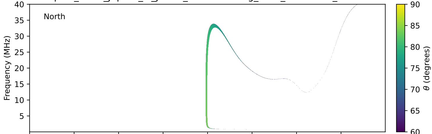
expres_earth_jupiter_io_jrm33_lossc-wid1deg_3kev_20120601_v11.cdf
