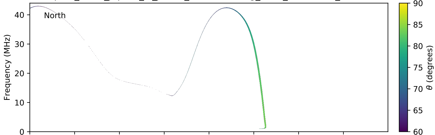
expres_earth_jupiter_io_jrm09_lossc-wid1deg_3kev_20120630_v01.cdf
