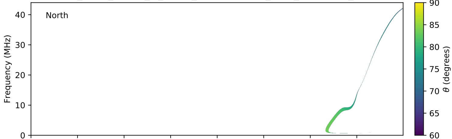
expres_earth_jupiter_io_jrm09_lossc-wid1deg_3kev_20120629_v01.cdf
