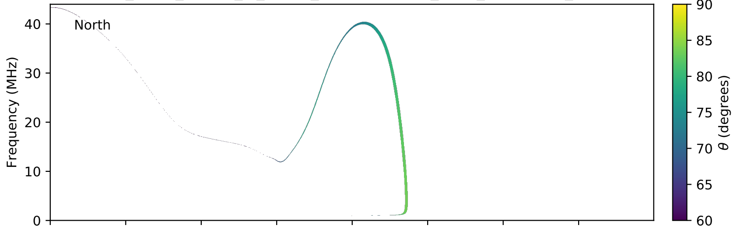
expres_earth_jupiter_io_jrm09_lossc-wid1deg_3kev_20120623_v01.cdf
