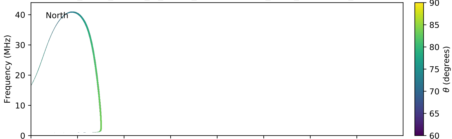
expres_earth_jupiter_io_jrm09_lossc-wid1deg_3kev_20120611_v01.cdf
