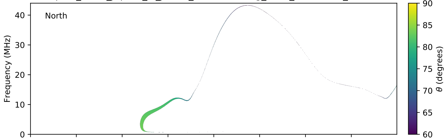
expres_earth_jupiter_io_jrm09_lossc-wid1deg_3kev_20120610_v01.cdf
