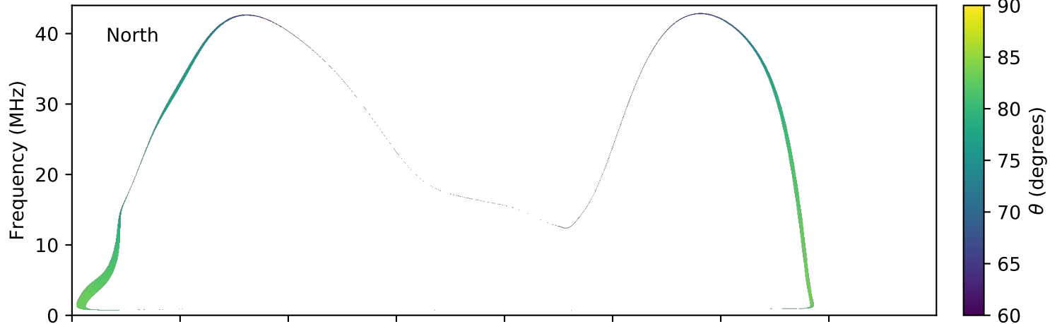
expres_earth_jupiter_io_jrm09_lossc-wid1deg_3kev_20120605_v01.cdf
