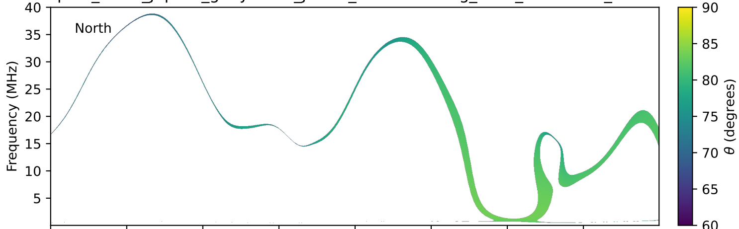
expres_earth_jupiter_ganymede_jrm33_lossc-wid1deg_3kev_20120618_v11.cdf
