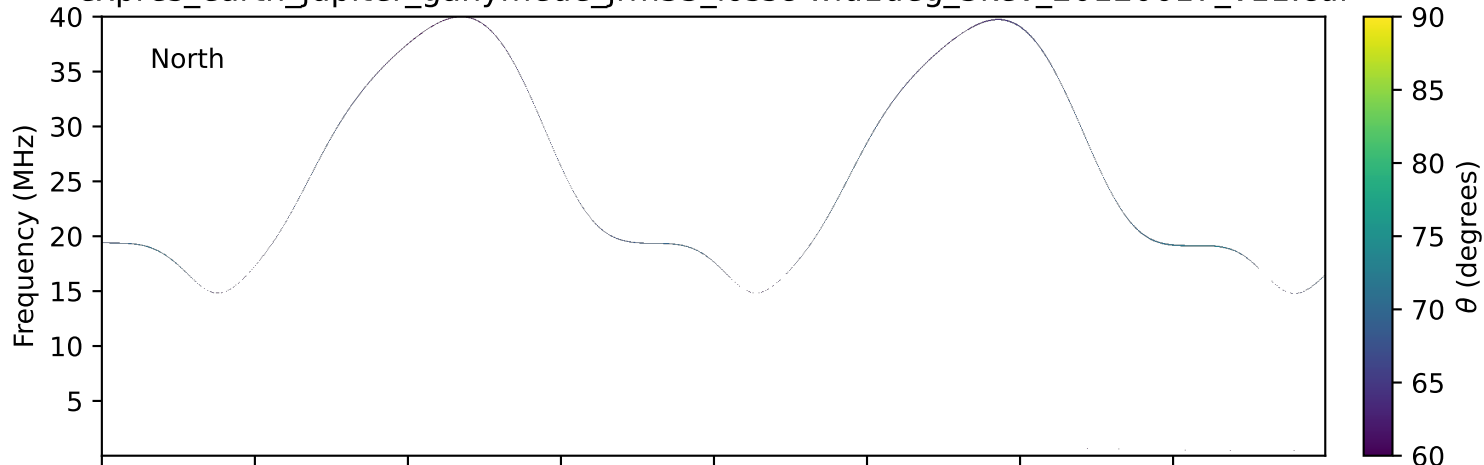
expres_earth_jupiter_ganymede_jrm33_lossc-wid1deg_3kev_20120617_v11.cdf
