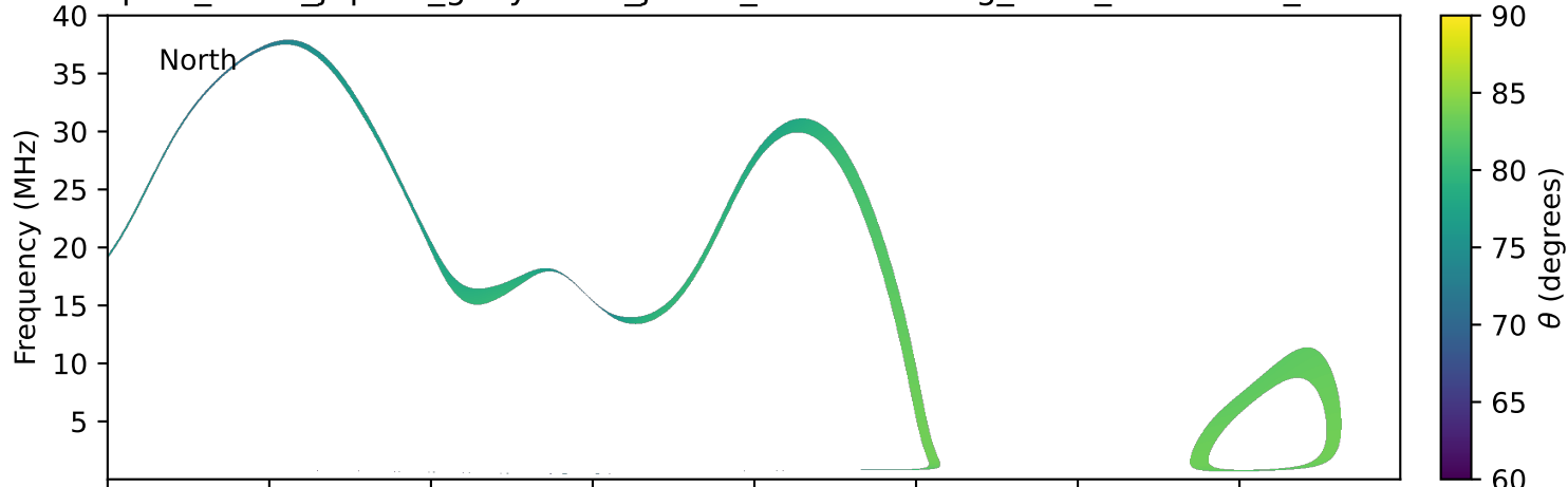
expres_earth_jupiter_ganymede_jrm33_lossc-wid1deg_3kev_20120611_v11.cdf
