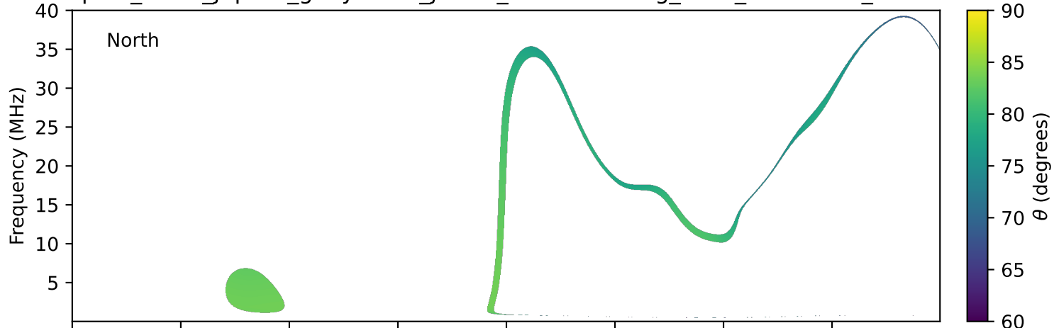
expres_earth_jupiter_ganymede_jrm33_lossc-wid1deg_3kev_20120608_v11.cdf
