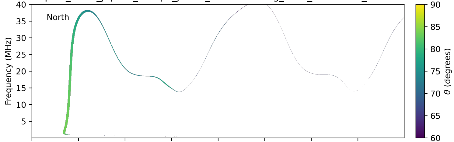
expres_earth_jupiter_europa_jrm33_lossc-wid1deg_3kev_20120615_v11.cdf
