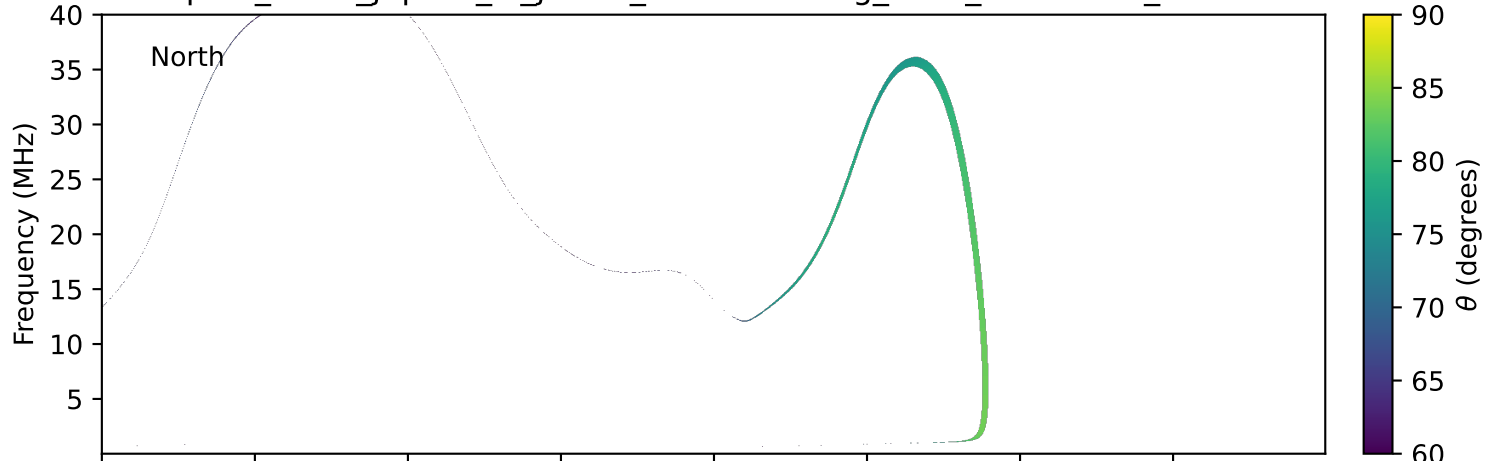
expres_earth_jupiter_io_jrm33_lossc-wid1deg_3kev_20120522_v11.cdf
