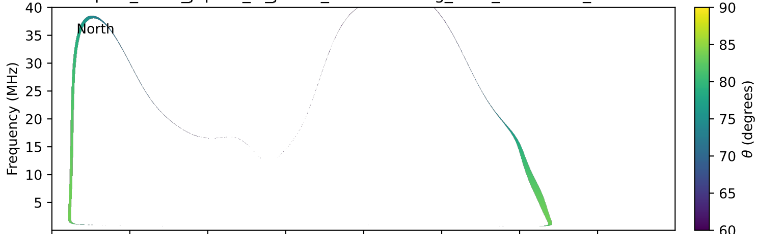
expres_earth_jupiter_io_jrm33_lossc-wid1deg_3kev_20120513_v11.cdf
