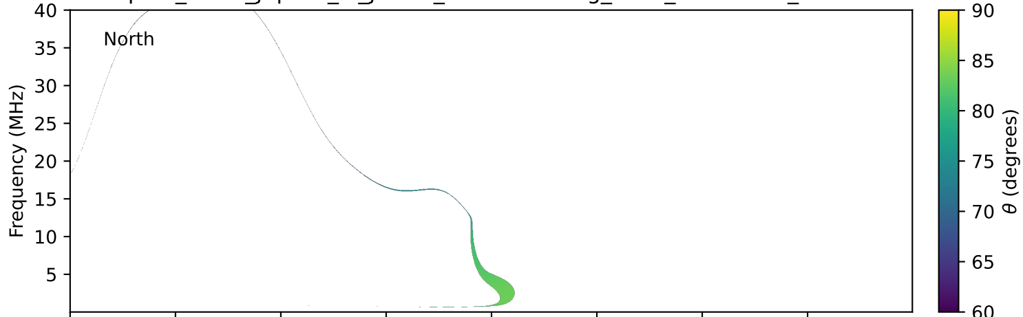
expres_earth_jupiter_io_jrm33_lossc-wid1deg_3kev_20120508_v11.cdf
