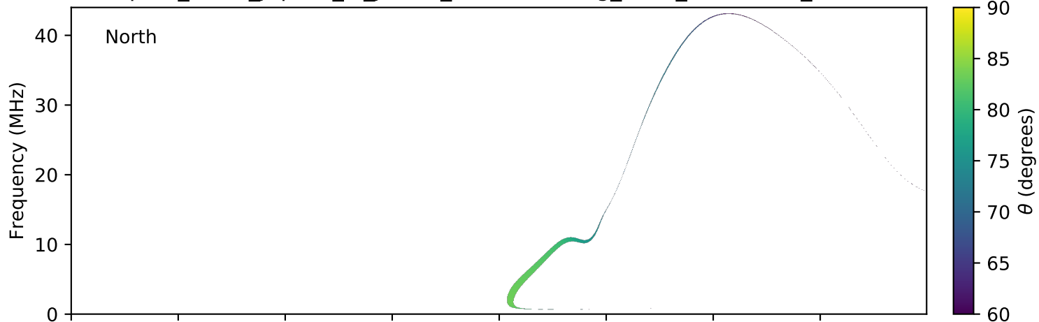
expres_earth_jupiter_io_jrm09_lossc-wid1deg_3kev_20120516_v01.cdf
