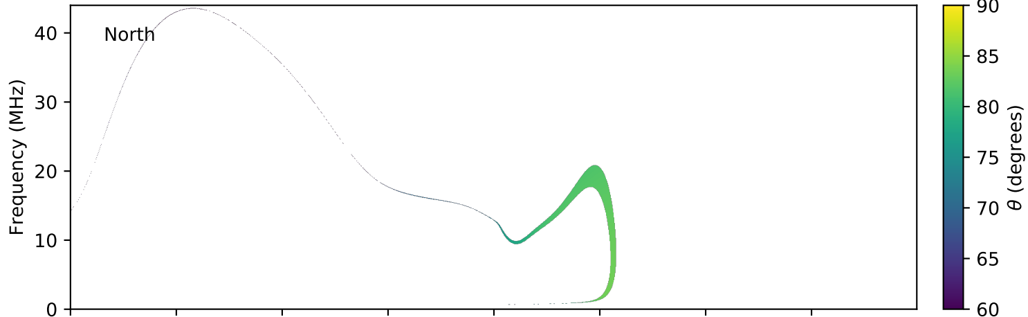
expres_earth_jupiter_io_jrm09_lossc-wid1deg_3kev_20120515_v01.cdf
