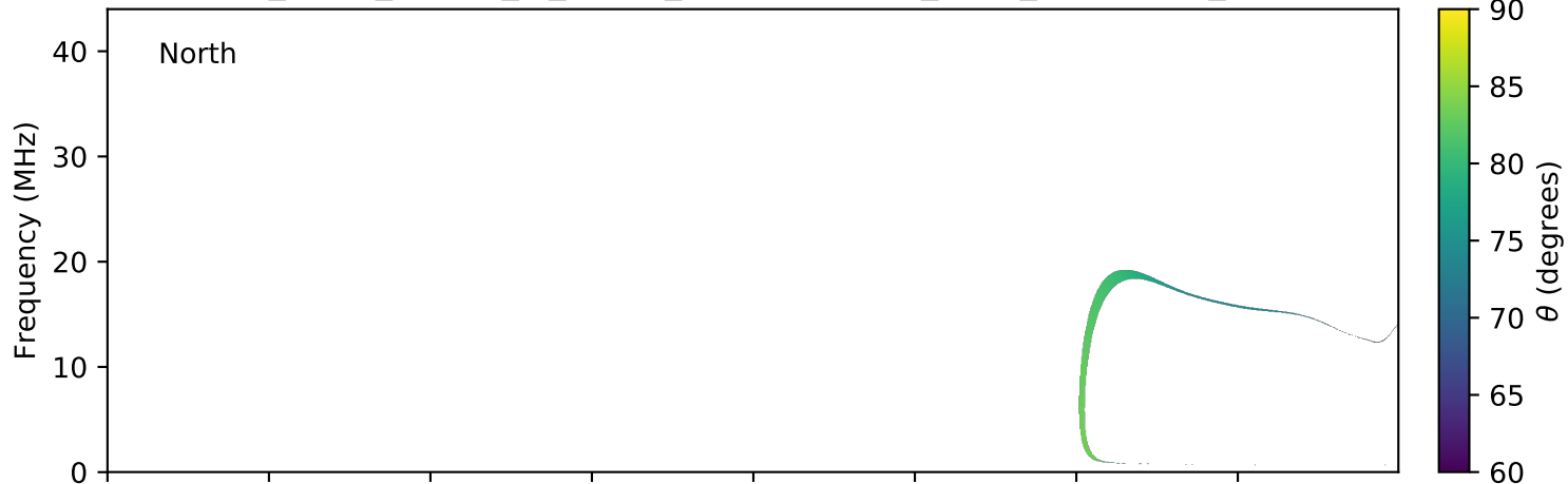
expres_earth_jupiter_io_jrm09_lossc-wid1deg_3kev_20120514_v01.cdf
