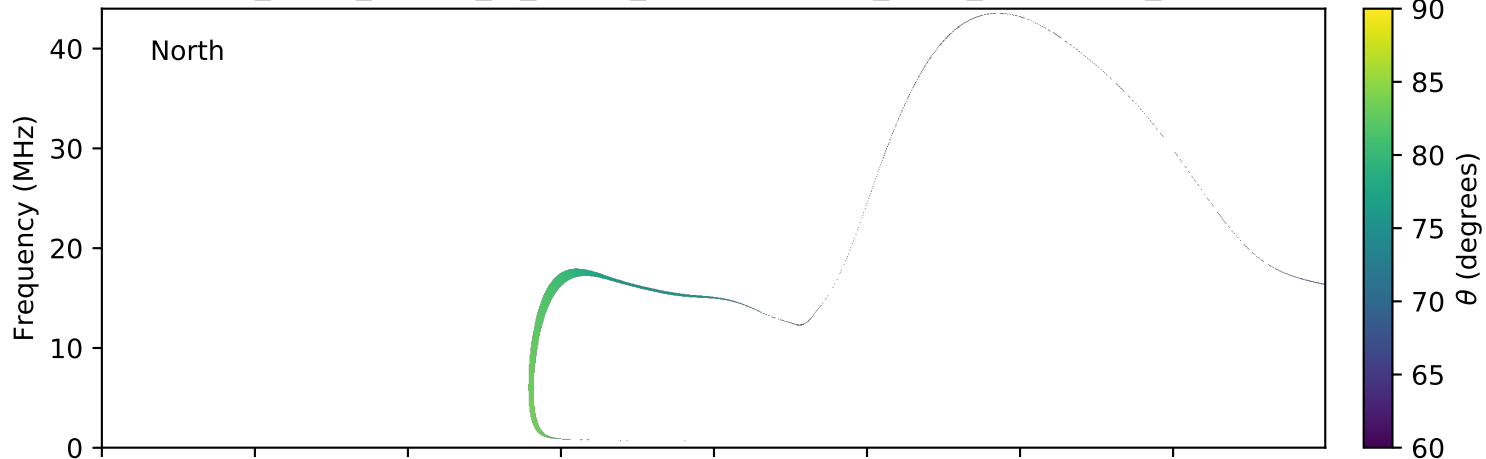
expres_earth_jupiter_io_jrm09_lossc-wid1deg_3kev_20120502_v01.cdf
