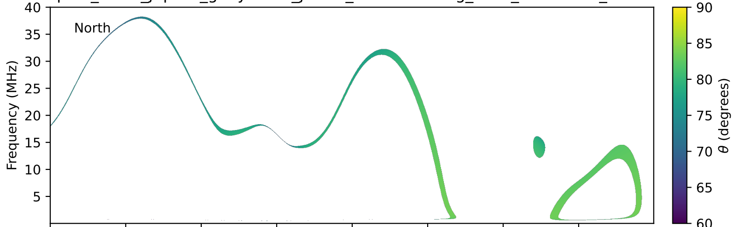
expres_earth_jupiter_ganymede_jrm33_lossc-wid1deg_3kev_20120506_v11.cdf
