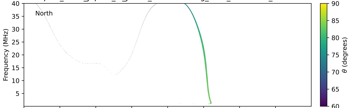
expres_earth_jupiter_io_jrm33_lossc-wid1deg_3kev_20120429_v11.cdf
