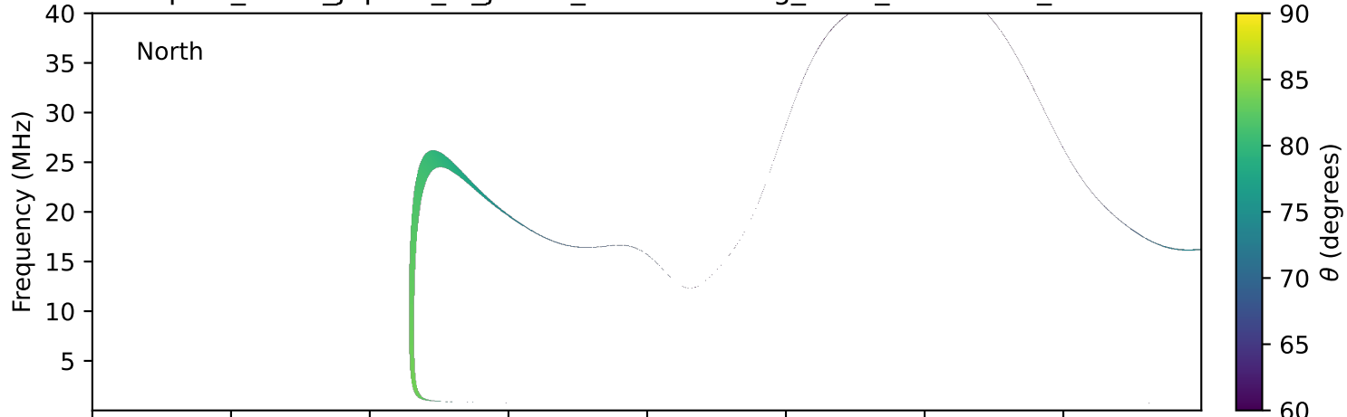
expres_earth_jupiter_io_jrm33_lossc-wid1deg_3kev_20120425_v11.cdf
