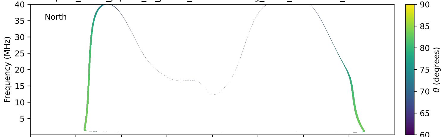
expres_earth_jupiter_io_jrm33_lossc-wid1deg_3kev_20120411_v11.cdf
