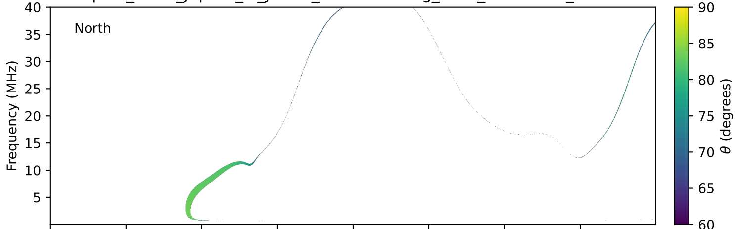
expres_earth_jupiter_io_jrm33_lossc-wid1deg_3kev_20120402_v11.cdf
