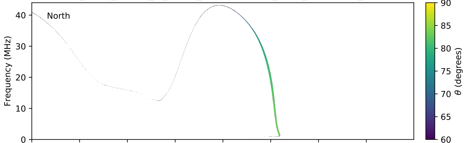
expres_earth_jupiter_io_jrm09_lossc-wid1deg_3kev_20120429_v01.cdf
