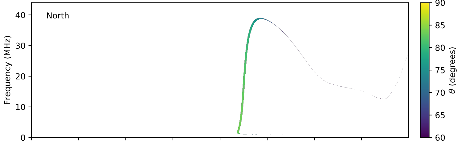
expres_earth_jupiter_io_jrm09_lossc-wid1deg_3kev_20120423_v01.cdf
