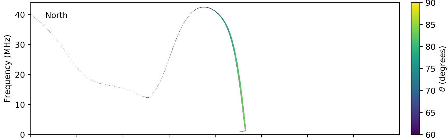
expres_earth_jupiter_io_jrm09_lossc-wid1deg_3kev_20120422_v01.cdf
