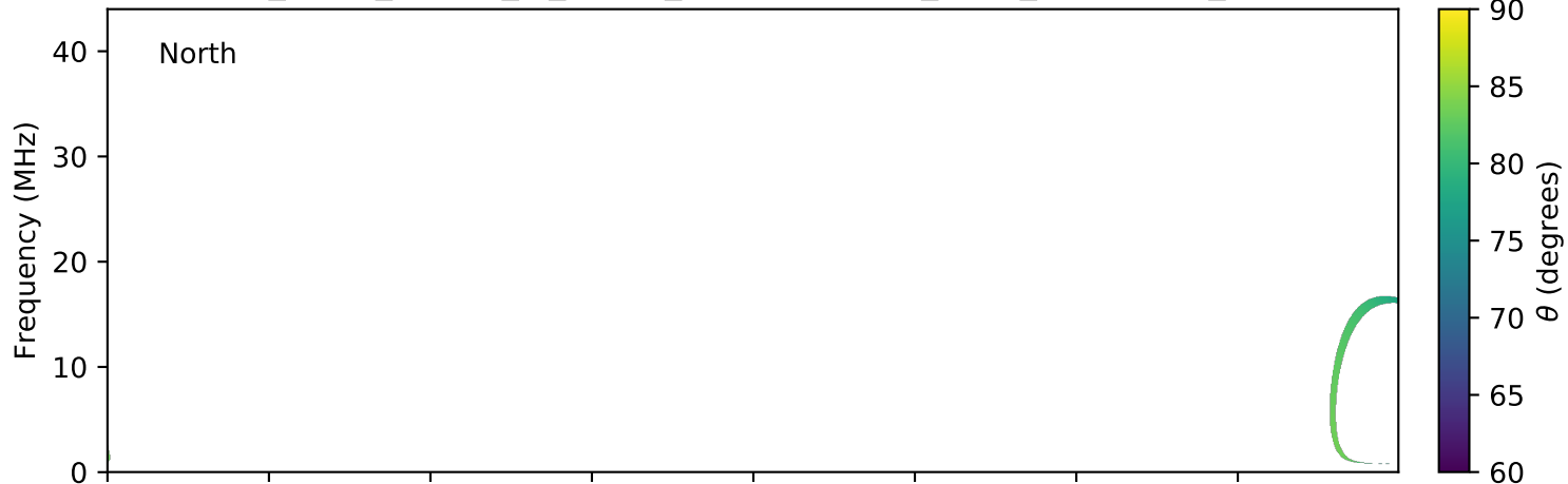
expres_earth_jupiter_io_jrm09_lossc-wid1deg_3kev_20120419_v01.cdf
