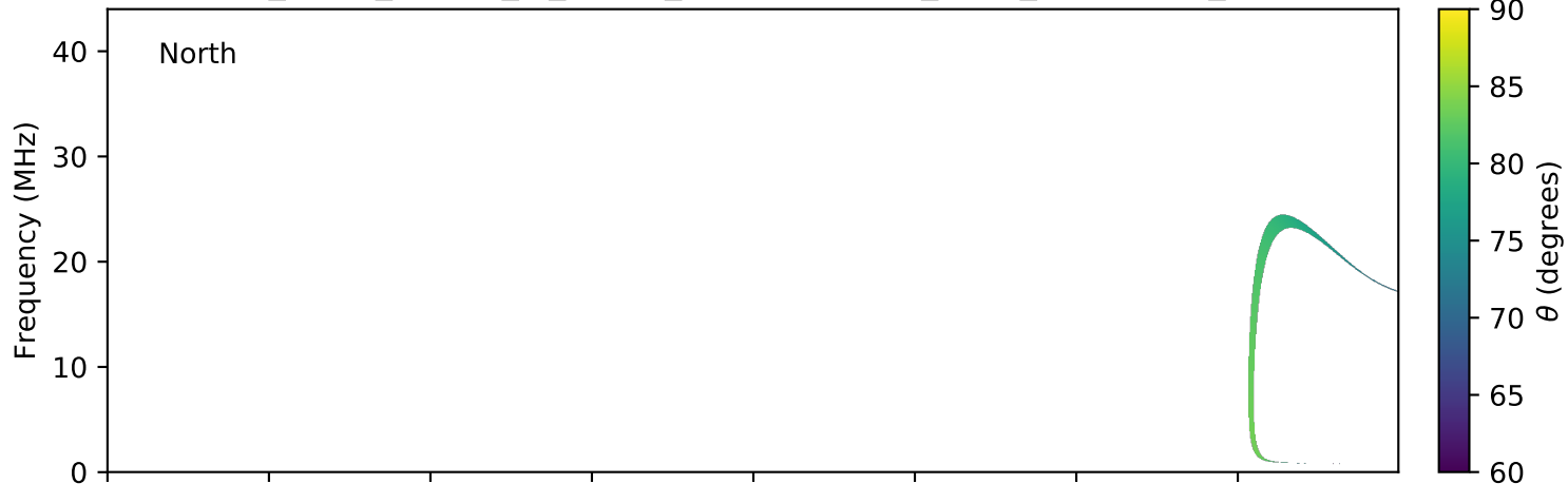
expres_earth_jupiter_io_jrm09_lossc-wid1deg_3kev_20120412_v01.cdf
