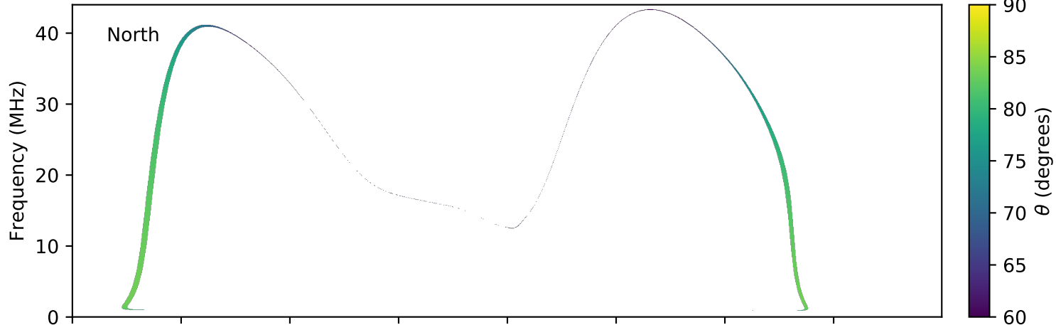
expres_earth_jupiter_io_jrm09_lossc-wid1deg_3kev_20120404_v01.cdf
