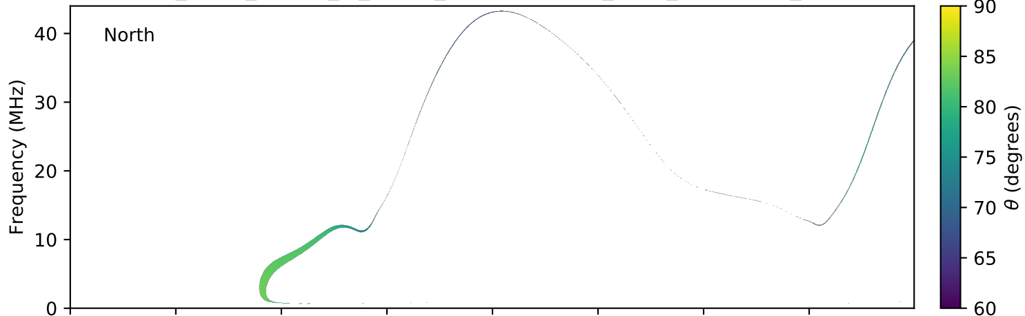
expres_earth_jupiter_io_jrm09_lossc-wid1deg_3kev_20120402_v01.cdf
