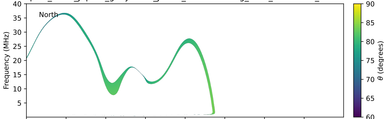
expres_earth_jupiter_ganymede_jrm33_lossc-wid1deg_3kev_20120429_v11.cdf
